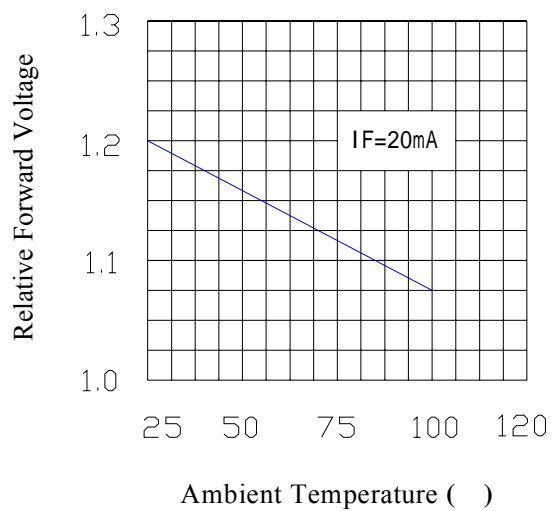
Fig.8 Forward Voltage vs. Ambient Temperature ( )
